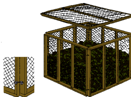
This bin with rain cover is very light and easy to store. The four side panels are connected with hooks and eyes
